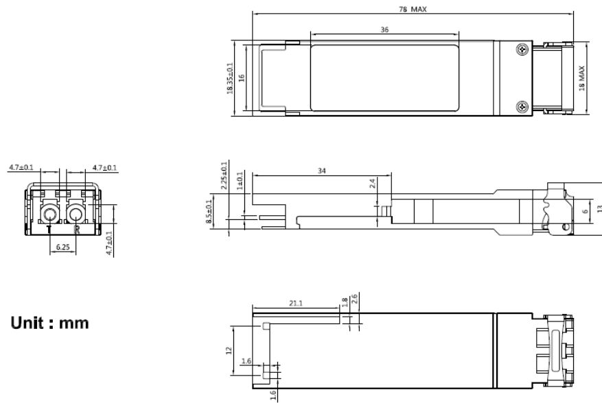
Figure 5. Outline Drawing
